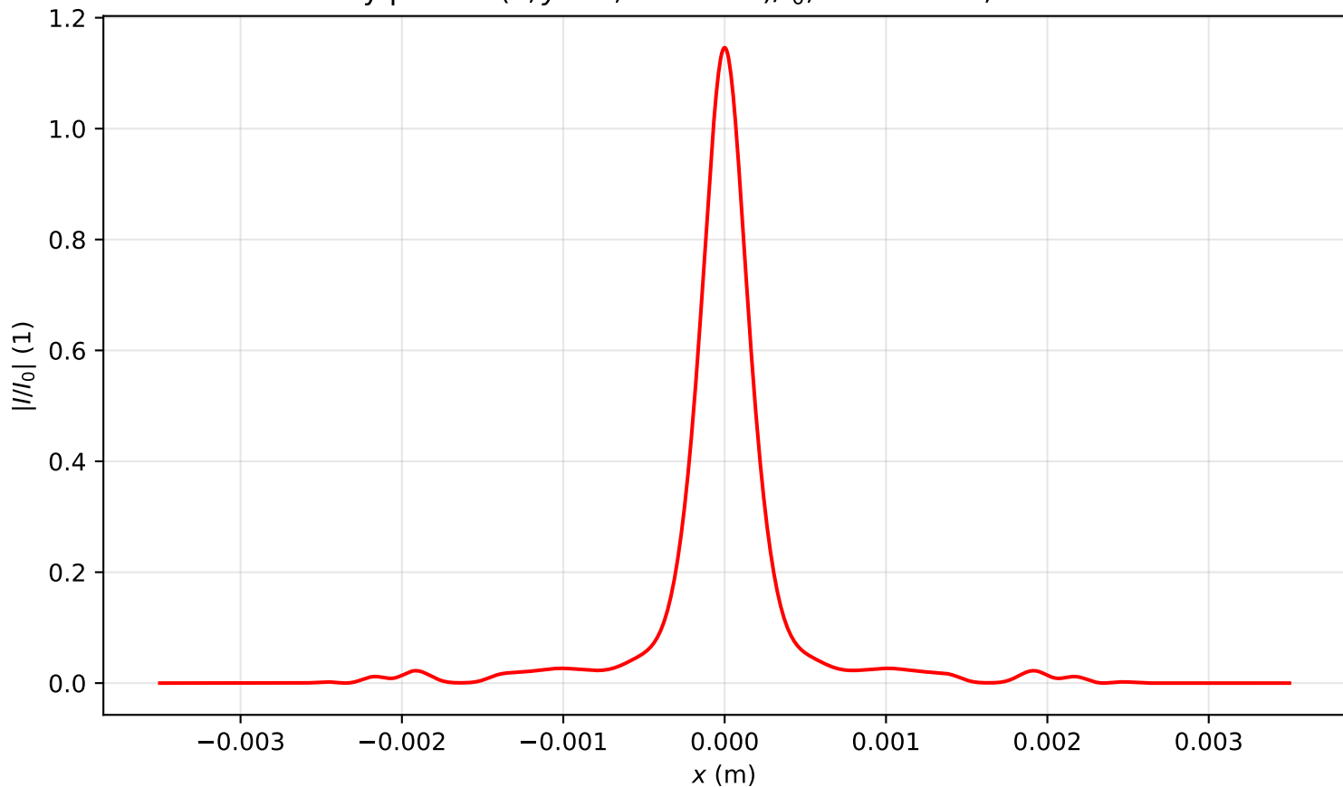
Intensity profile I(x, y = 0, z = 3.344)/I_0 , P_{in}=4.0P_{cr} , artificial time
